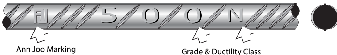
D500N Straight Bar (From 1 May 2018)
