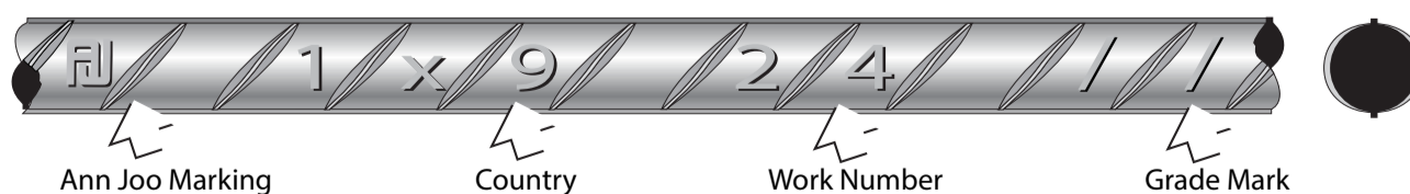
D500N Straight Bar (From 1 May 2018)
