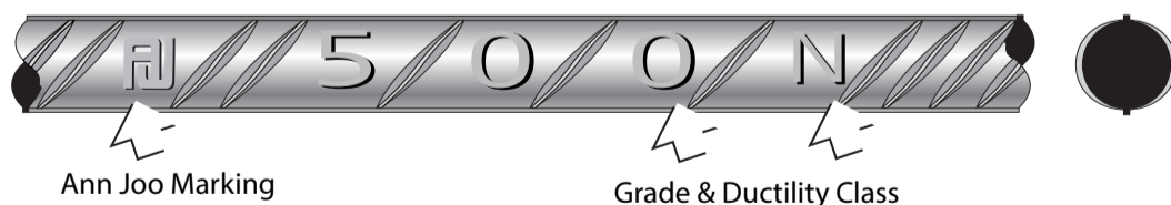
D500N Straight Bar (From 1 May 2018)
